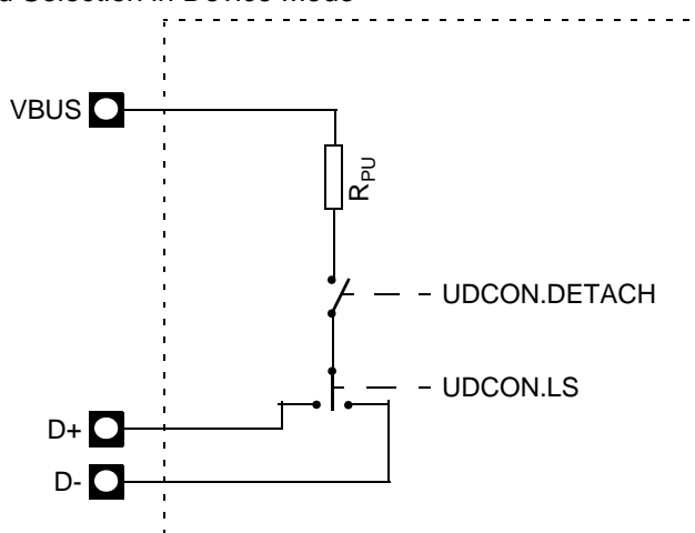
Figure 22-7. Speed Selection in Device Mode
